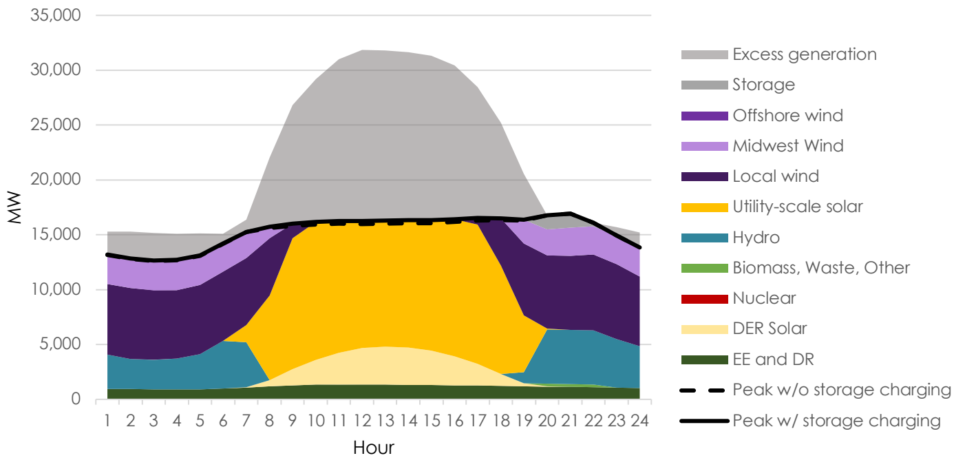
TVA, LSR-FOCUSED CES, SPRING DAY, 2035
