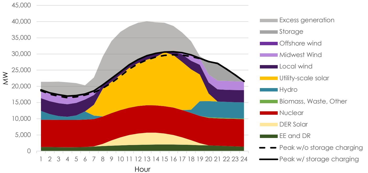
TVA, LSR-FOCUSED CES, SUMMER PEAK DAY, 2035
