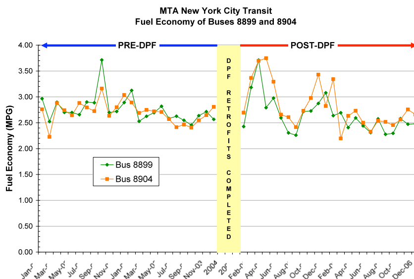
Figure 3: Monthly Fuel Economies for Two NYC Transit Buses (Source: M. J. Bradley & Associates.)
