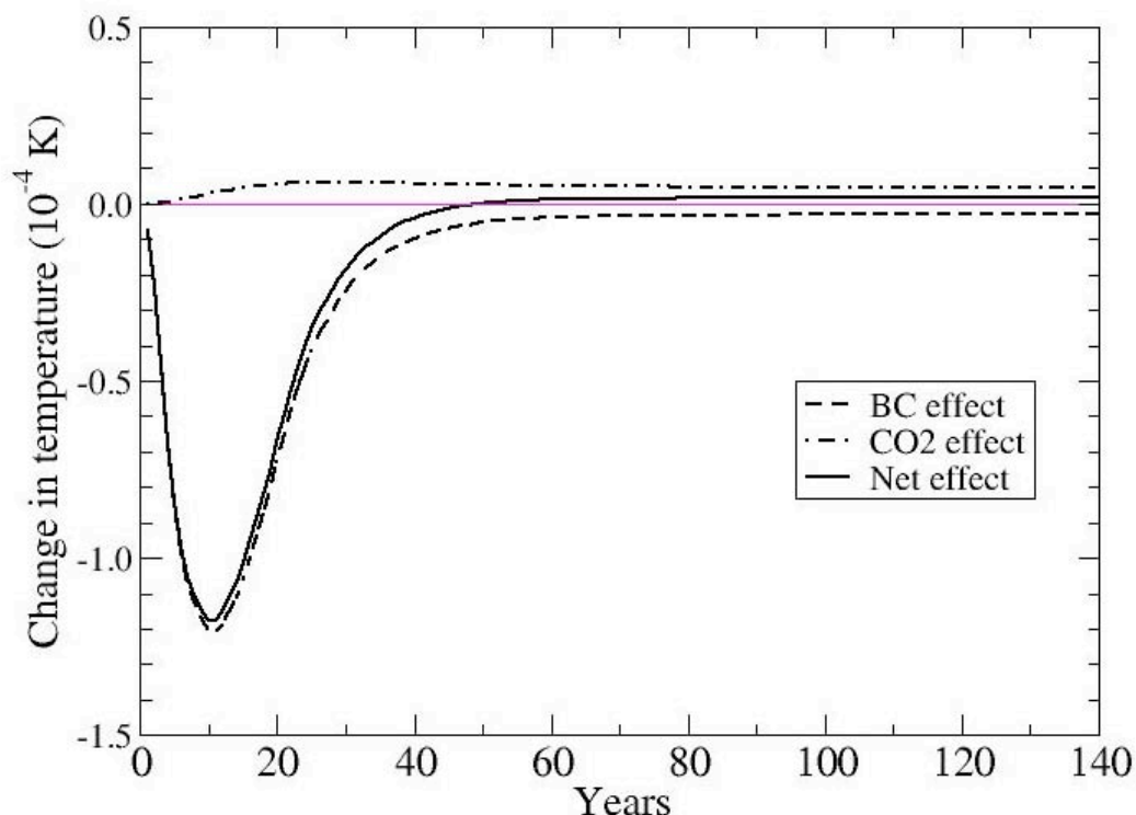
Figure 6. Modeled GTP-based benefits a CATF-proposed class 8 truck rebuild rule in the U.S., assuming a 2 percent fuel penalty, courtesy, Olivier Boucher, Hadley Centre, UK (2009). The net CO 2 e reduction benefit lasts about half a century followed by a very small CO 2 warming as a result of the fuel penalty.
