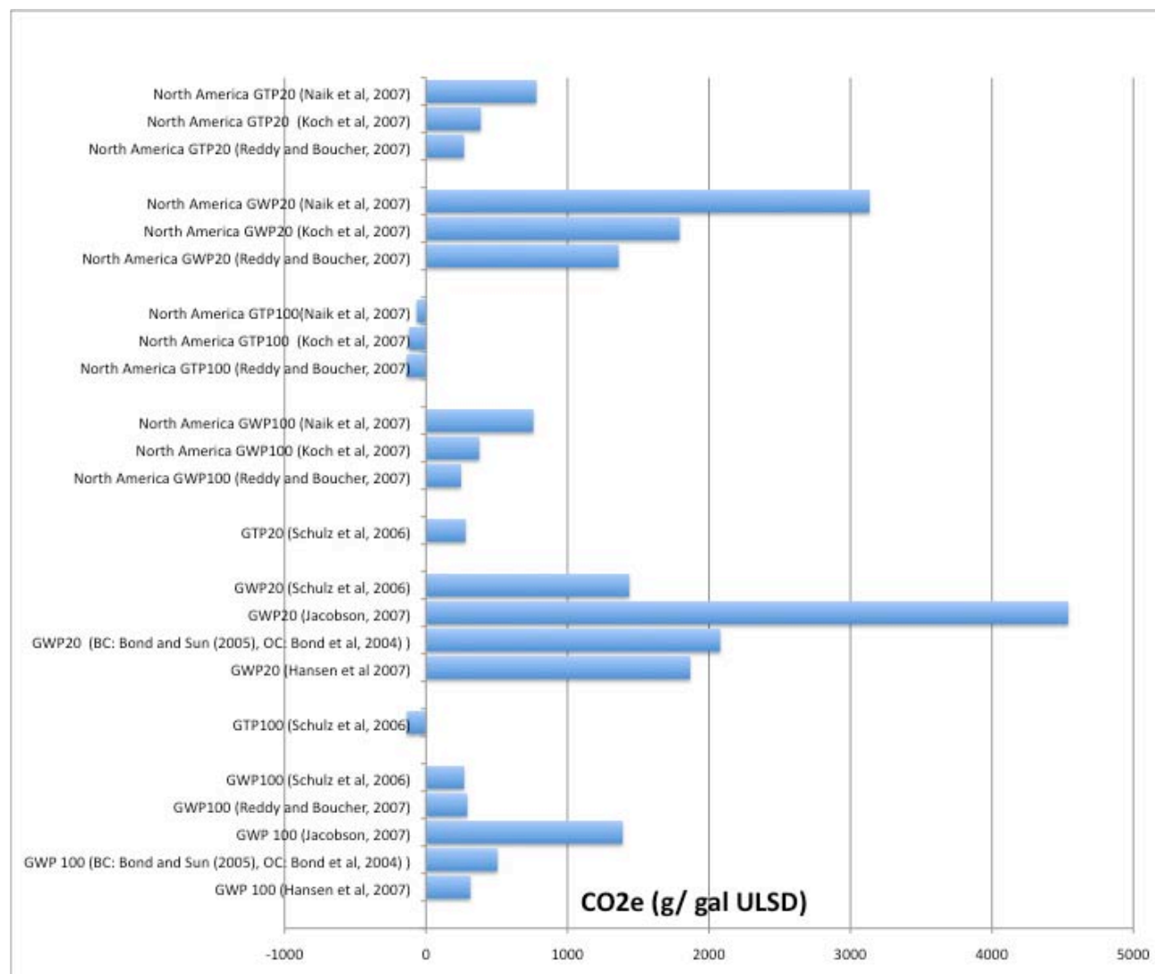
Figure 4: Ranges of black carbon CO 2 e benefits (g/gal) for the DPF retrofit of a U.S. class 8 truck, assuming a 2 percent fuel penalty.
