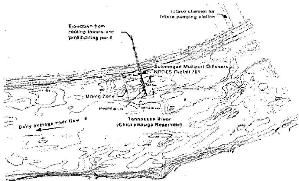
Figure 3-1. Mixing Zone for Outfall 101
